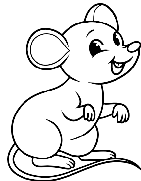
mouse
