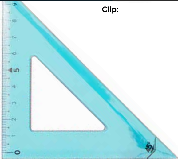
Triangle:
