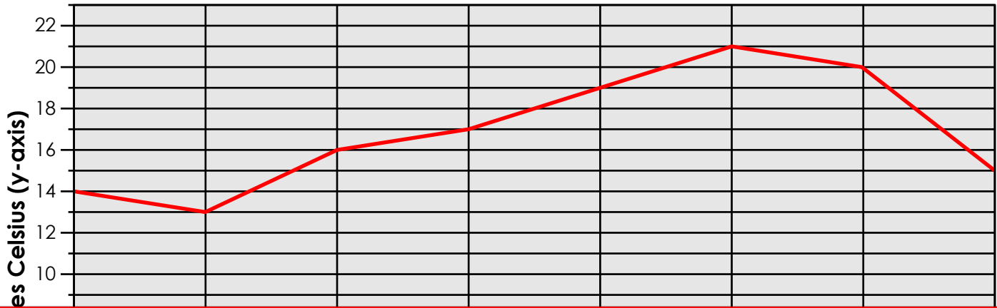
Air Temperature on Wednesday
