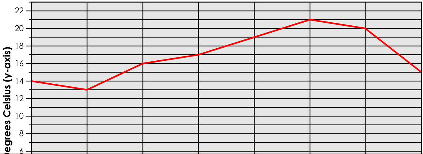
Air Temperature on Wednesday
