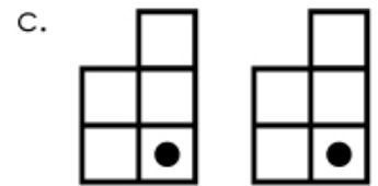
translation
