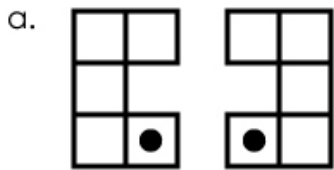
reflection
