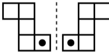
REFLECTION
