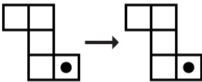
TRANSLATION
