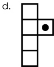
translation
