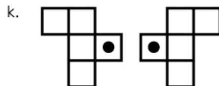
reflection
