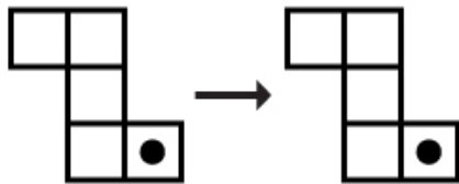
TRANSLATION
