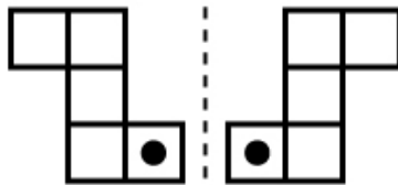
REFLECTION
